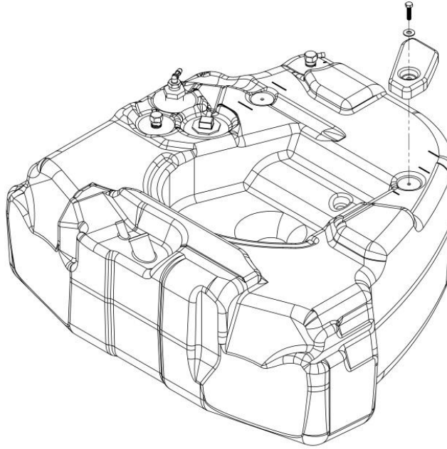
(Fig. 9) Exploded view showing spacer (02 0000 0170) required on 05--07 Ford attaches to chassis frame
