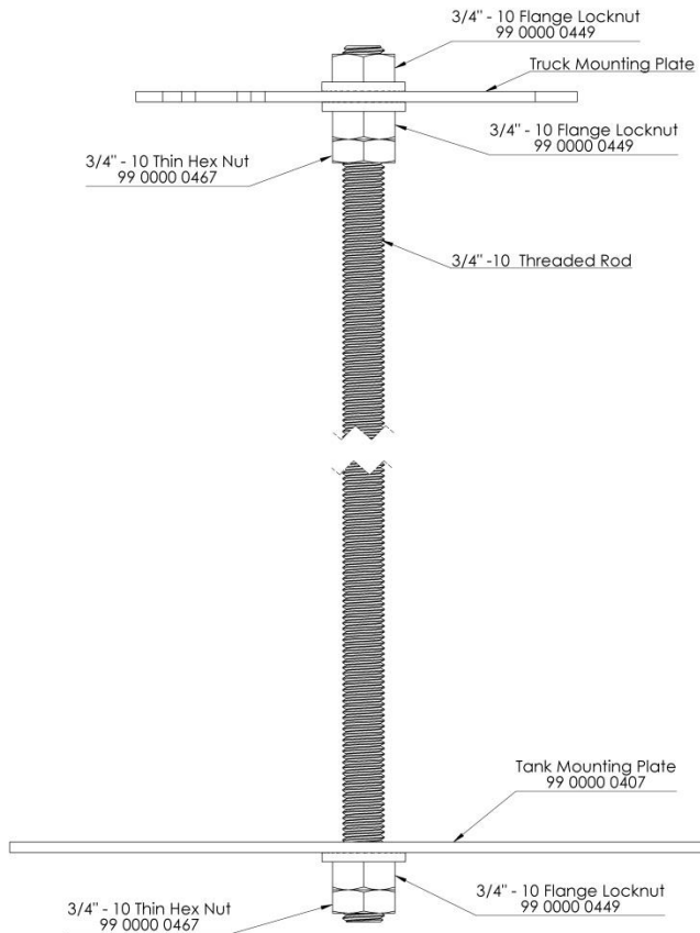
(Fig. 4) Side view of tank mounting plate assembly, threaded rod, and bottom tank mounting plate. Be sure to torque the nuts on the top plate to 45 ft. lbs, the flanged nut on underside of Tank Mounting Plate to 15 ft. lbs. against the tank and the jam nuts ("Thin Hex Nut") at the plate and very bottom to 45 ft. lbs.
