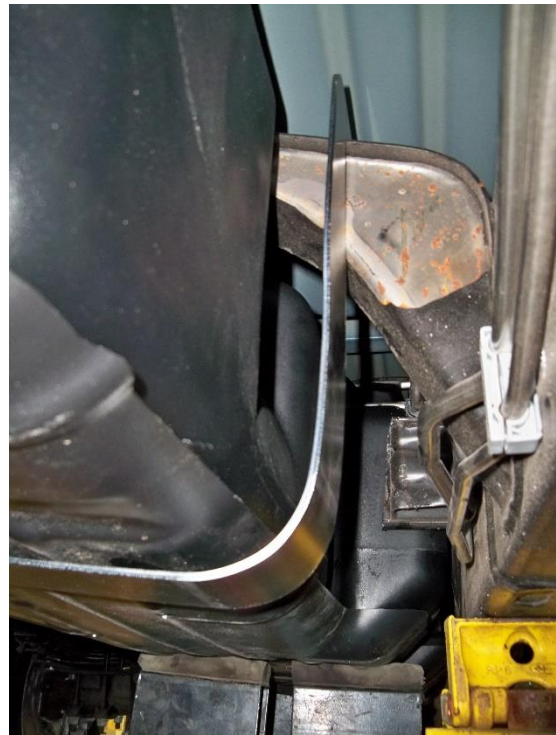
(Fig. 15) Hanger Bracket installed on frame
