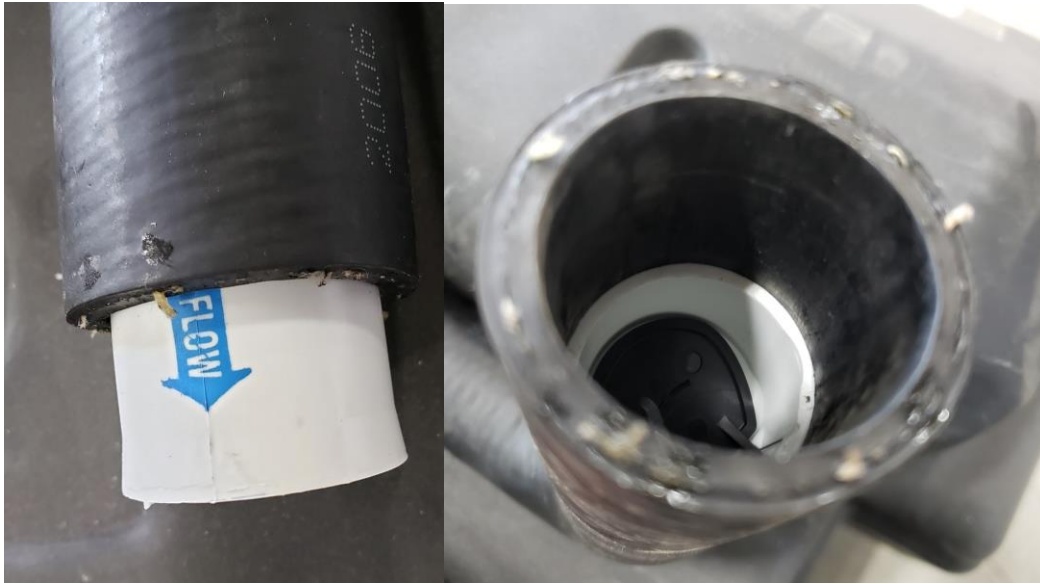
(Fig. 11) Insert 1-1/2" Fill Pipe ICV into fill hose with the "Flow" arrow pointing towards the fuel tank. This will need to be inserted deep enough to allow the fill hose to fit completely over the king nipple.
