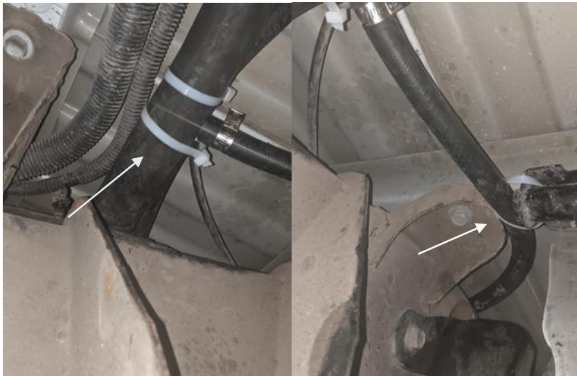
(Fig. 10) Zip tie the hose into place to prevent it from sagging in the future. Zip tie the tee to the top of the filler neck hose. Tighten all hose clamps appropriately.
